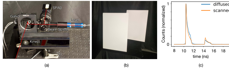
Fig. 4: (a) Prototype scanning setup. The pulsed light from the laser travels through a beam splitter before being guided by the galvo to the scene. Returning light is measured by the single-pixel SPAD. The Kinect v2 RGB camera is used to capture the image used to generate the monocular depth estimate (the depth camera is not used). (b) Scene and (c) measurements for diffused and summed scanned mode (10s capture, aligned peaks). The observed counts in the diffuse mode match closely with the sum of the raster-scanned measurements.
