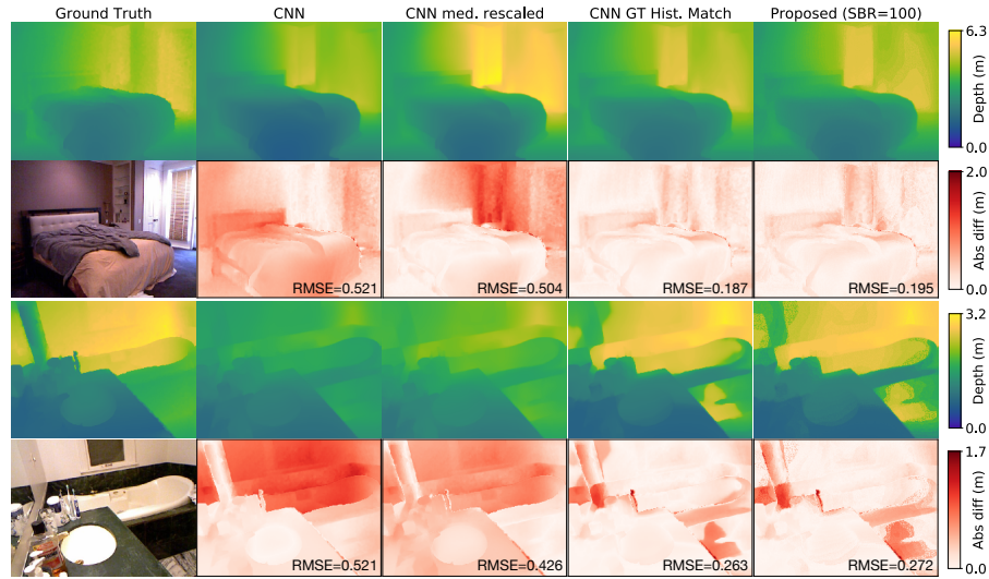
Fig. 3: Simulated results from NYU Depth v2 computed with the DenseDepth CNN [2]. The depth maps estimated by the CNN are reasonable, but contain systematic error. Oracle access to the ground truth depth maps, either through the median depth or the depth histogram, can remove this error and correct the depth maps. The proposed method uses a single transient measurement and does not rely on ground truth depth, but it achieves a quality that closely matches the best-performing oracle.
