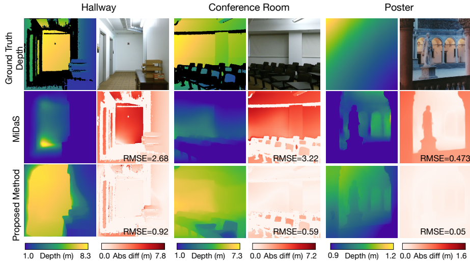
Fig. 5: Experimental results. For each scene, we record a ground truth depth map that is raster-scanned with the SPAD (upper left subimages), and an RGB image (upper right subimages). A monocular depth CNN predicts an initial depth map (top middle left subimages), which is corrected with the digitally aggregated SPAD histogram using the proposed method (bottom left subimages), as shown by the error maps and root mean squared error (RMSE) for each example (middle left, bottom subimages). The CNN is confused when we show it a photograph of a poster (rightmost scene); it incorrectly predicts the depth of the scene depicted on the flat print. Our method is able to correct this error.
