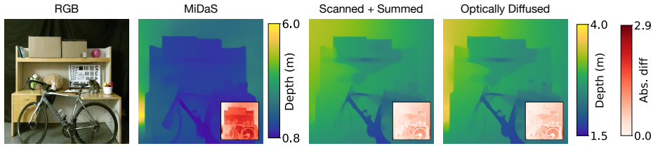
Fig. 6: Captured result comparing the direct output of the MiDaS MDE and depth maps corrected by our method using the digitally aggregated transient of the scanned SPAD (center right) and a single transient captured by an optically diffused SPAD and laser (right). Both of these approaches result in very similar results and both are significantly better than the output of the MDE, as shown by the error maps in the insets. The diffused SPAD results are captured at \sim 25\text{mW} laser power indoors.
